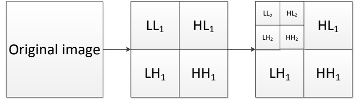
Fig. 2 wavelet decomposition
