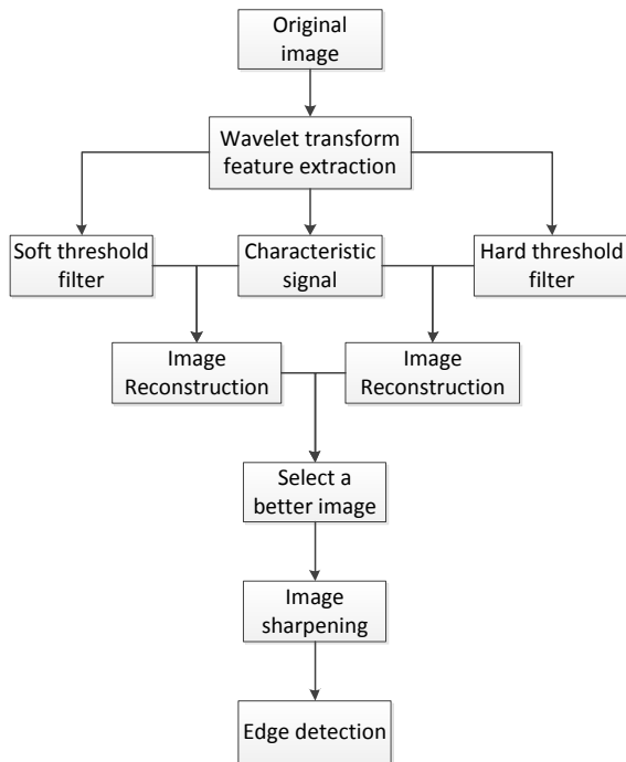
Fig. 3 The flow chart of edge detection based on wavelet de-noising
