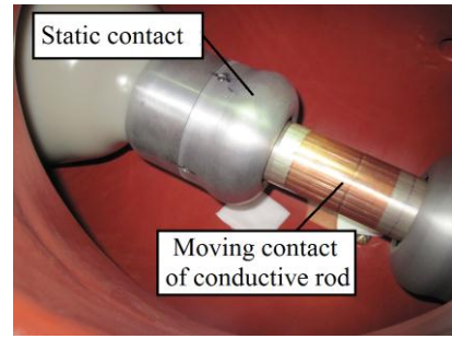
Fig. 4 The conductive rod in GIS tank
