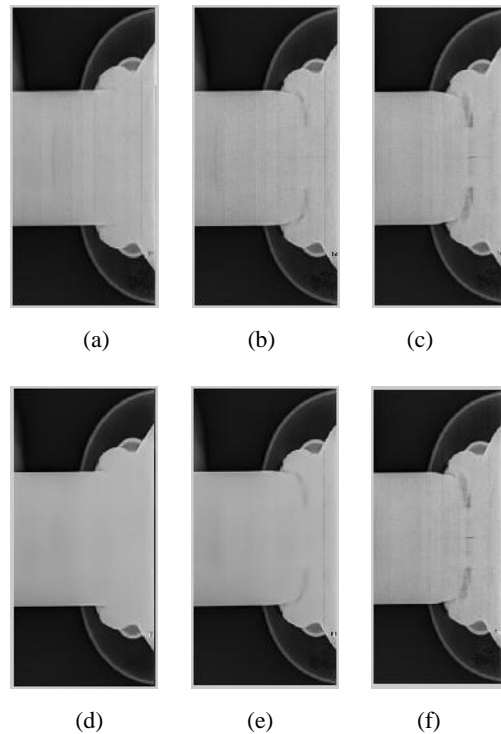
Fig. 8 the comparison chart with wavelet de-noising and sharpening
